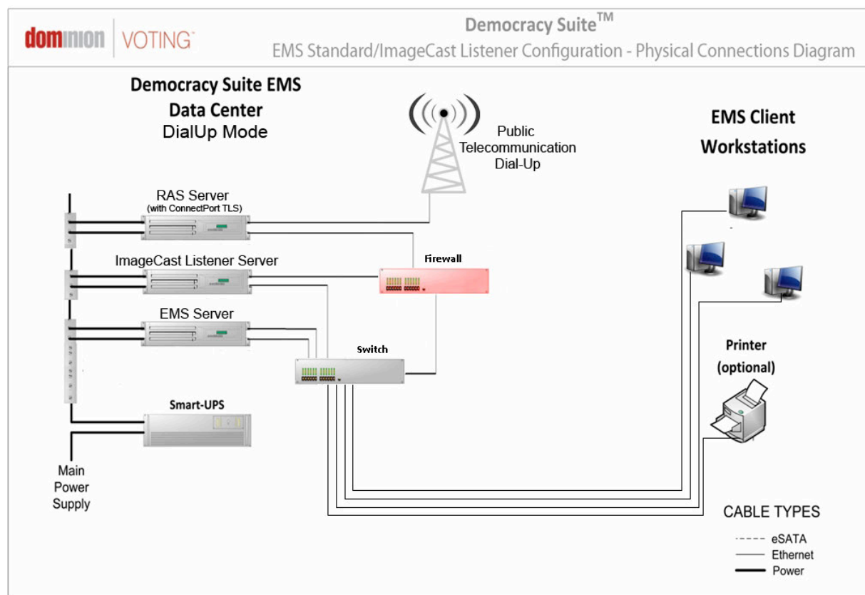
Figure 3.6: The EMS Standard/ImageCast® Listener Dial-up Configuration: Physical Connections
