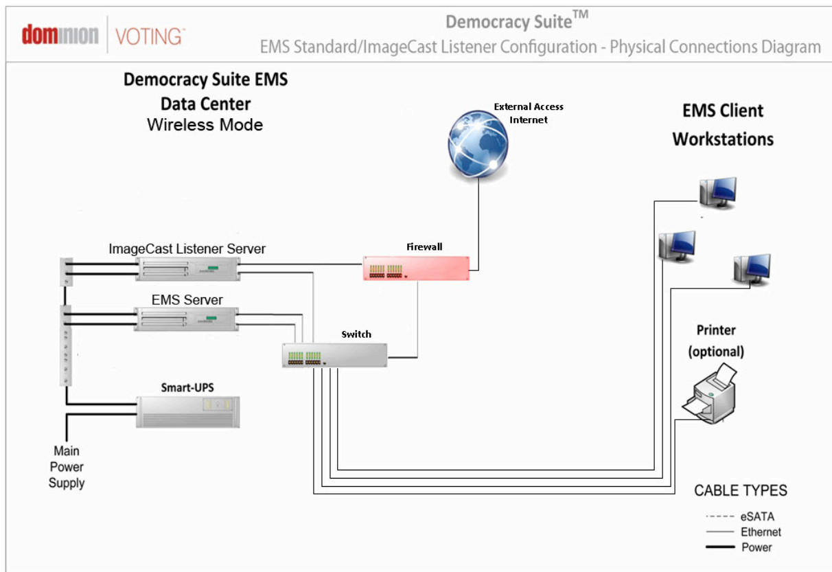
Figure 3.5: The EMS Standard/ImageCast® Listener Wireless Configuration: Physical Connections
