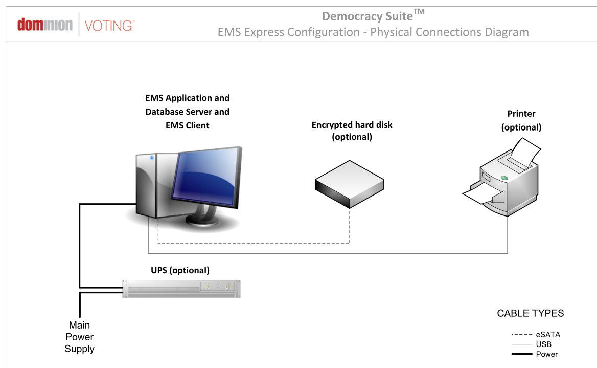
Figure 3.2: The Democracy Suite® EMS Express Configuration - Physical Connections.
